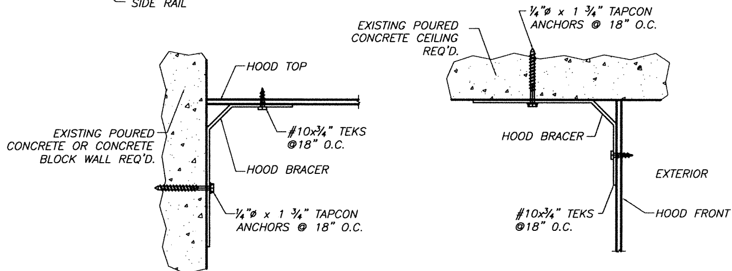
WALL HOOD ATTACHMENT (SIDE VIEW)
