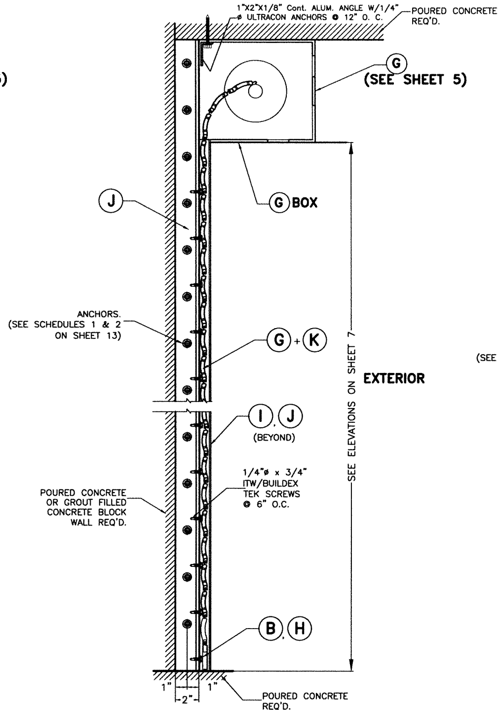
CASES I, II, III & IV SECTION B-B (TRAPPED MOUNTED) SCALE 1-1/2"=1"
