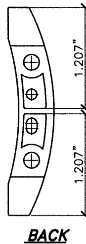
K ACETAL POLYMER (Fu=9.5Ksl., 110 DUROMETER) END RETAINER CAP
