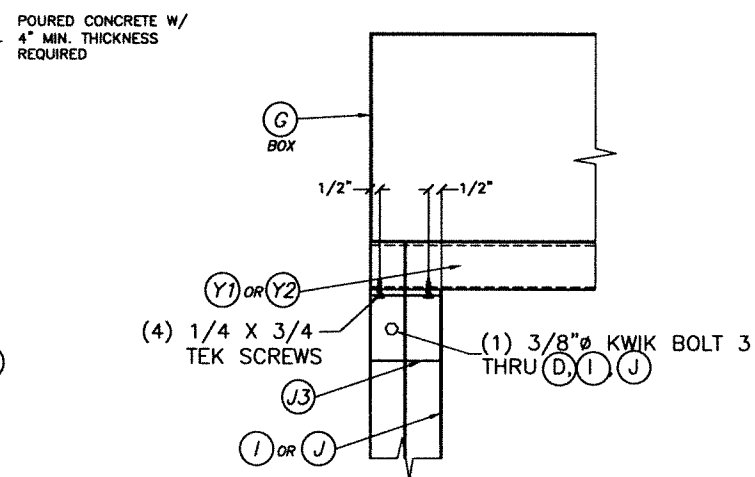
(2) (J4) W/ (4) 1/4" Ø THRU BOLT TO HEADER & (2) 3/8" Ø KWIK BOLT 3 W/ 2 1/2" Min. EMBEDMENT TO WALL.
