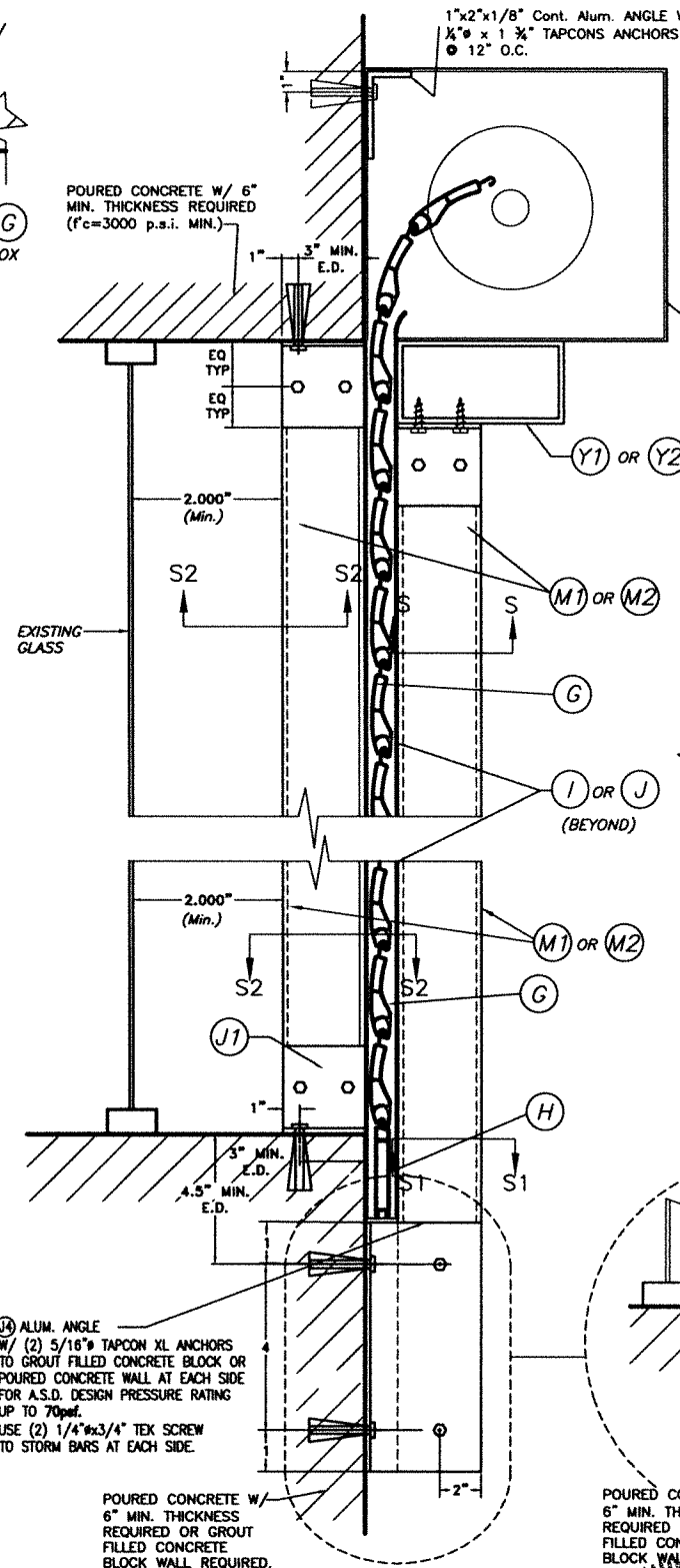
WALL MOUNTING SECTION D-D INSTALLATION W/ FIXED STORM BARS W/ CONCRETE ANCHORS SCALE : N.T.S
