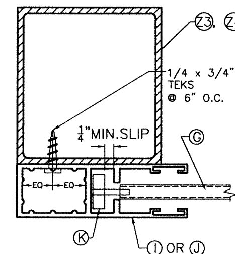
SECTION J''-J'': MULLION MOUNT (FACE MOUNT)
